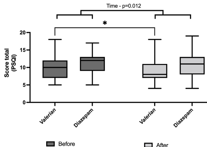
Figure 2: PSQI_total score.
